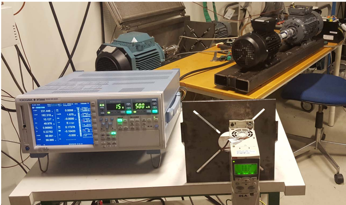
Test set up with converter, converter-fed motor, load motor and measuring instrument
